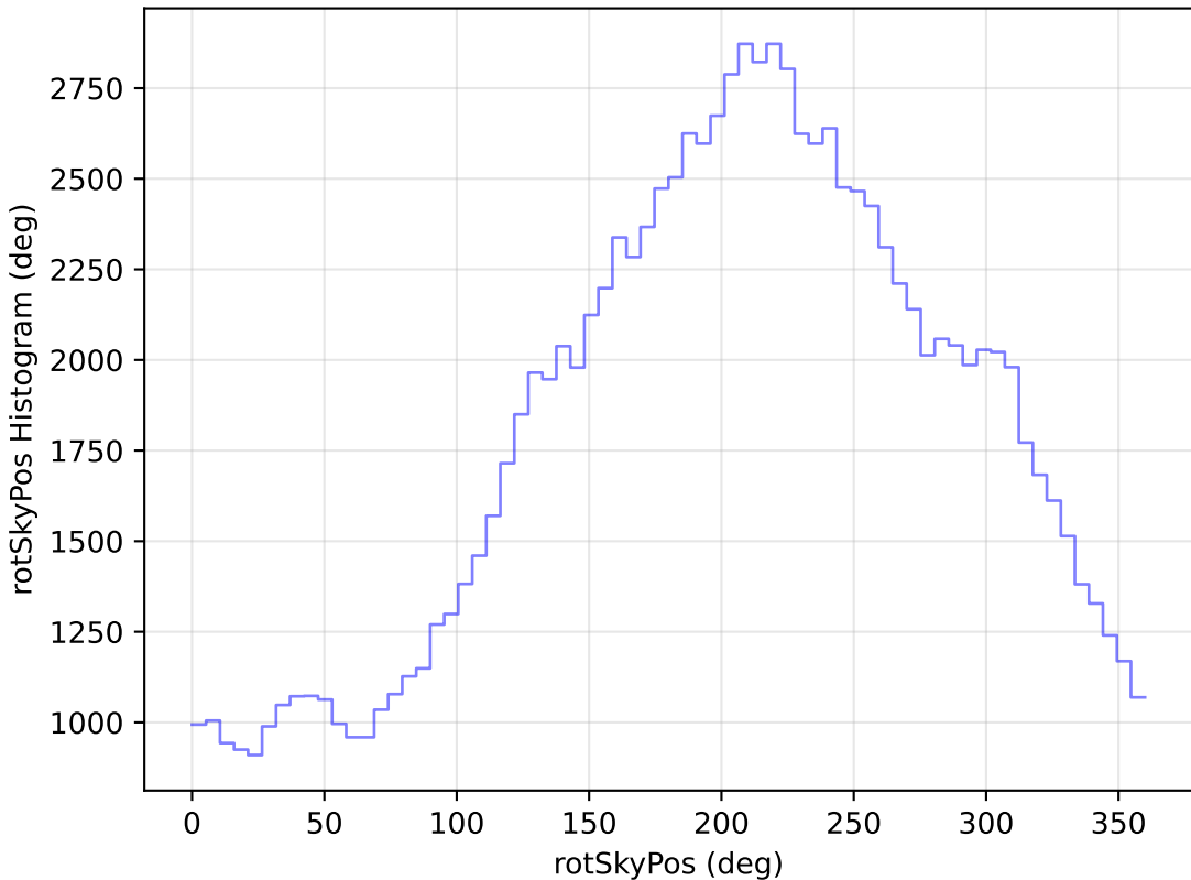
too_elab_r64_d2_griz_v3.4_10yrs All sky u band: rotSkyPos Histogram
