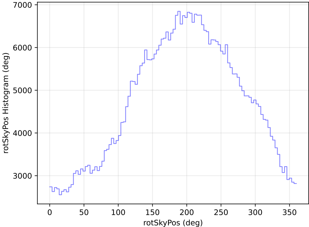
too_elab_r64_d2_griz_v3.4_10yrs All sky r band: rotSkyPos Histogram
