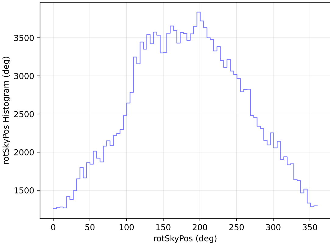
too_elab_r64_d2_griz_v3.4_10yrs All sky g band: rotSkyPos Histogram
