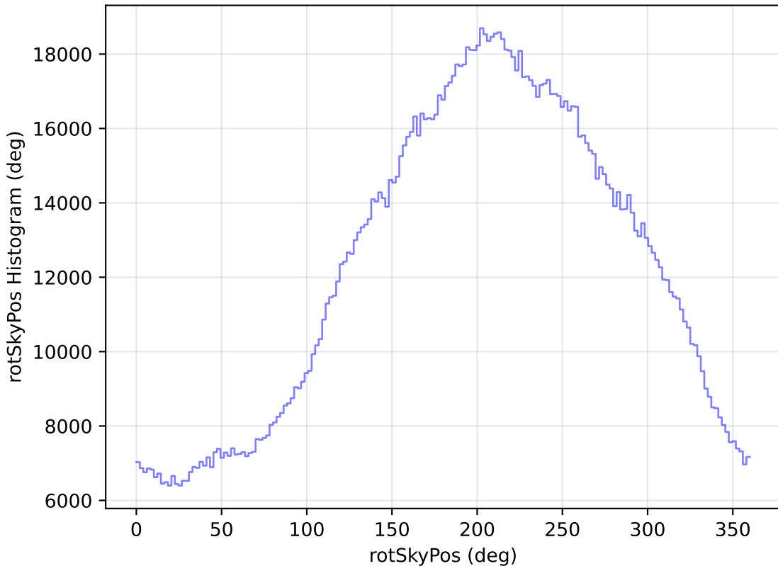
too_elab_r64_d2_griz_v3.4_10yrs All sky all bands: rotSkyPos Histogram
