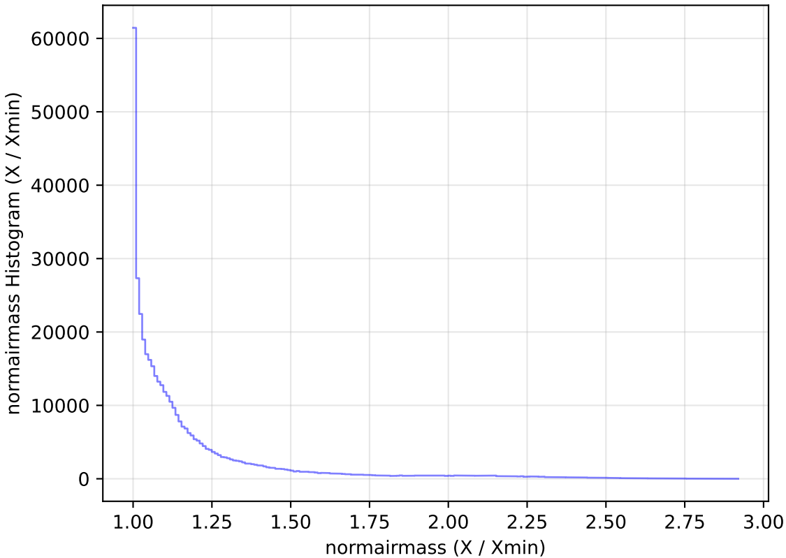
too_elab_r64_d2_griz_v3.4_10yrs WFD z band: normairmass Histogram
