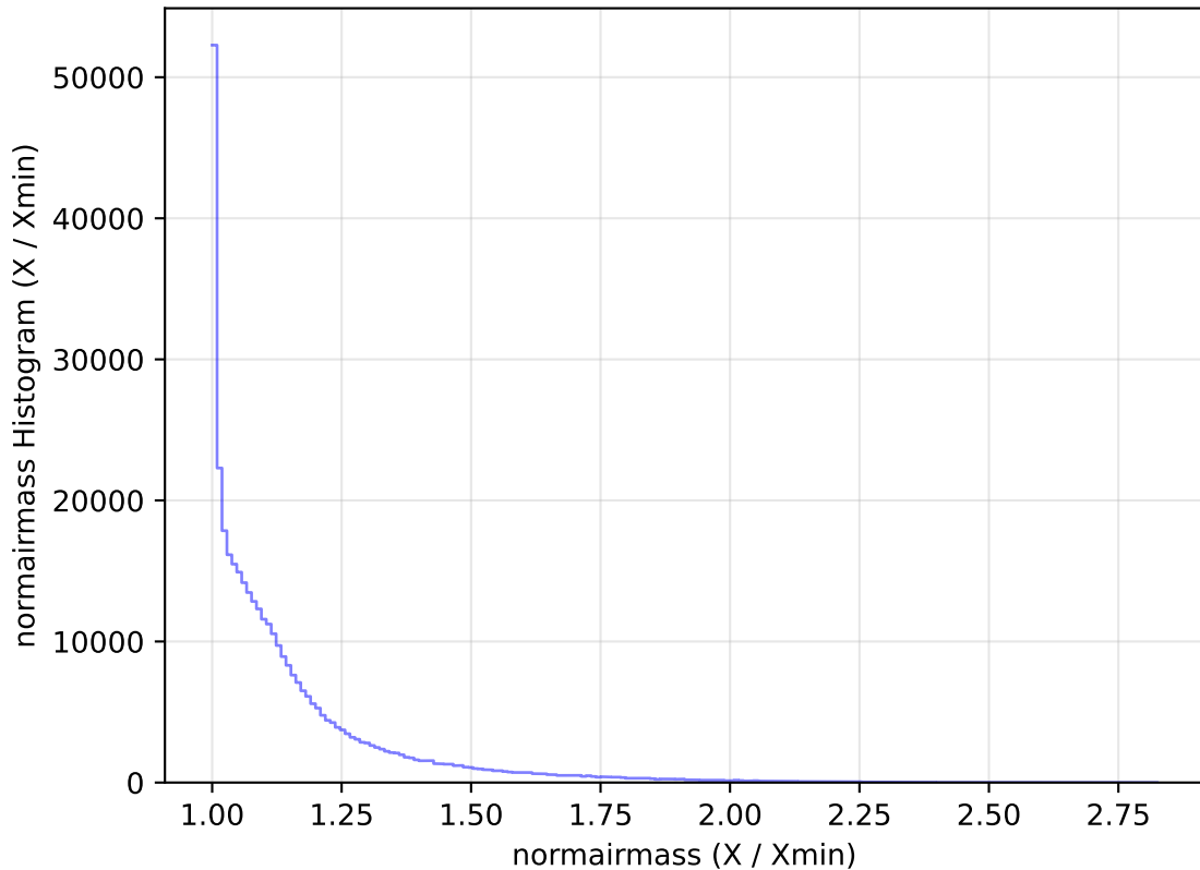
too_elab_r64_d2_griz_v3.4_10yrs WFD y band: normairmass Histogram
