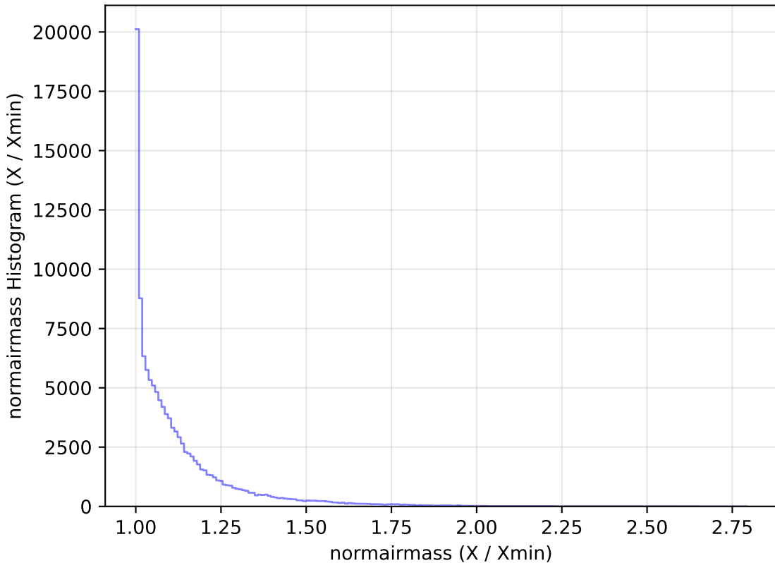
too_elab_r64_d2_griz_v3.4_10yrs WFD u band: normairmass Histogram
