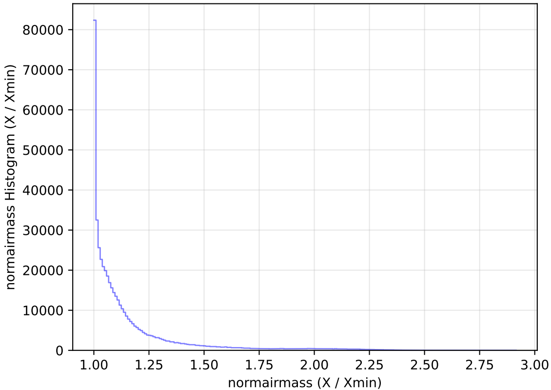
too_elab_r64_d2_griz_v3.4_10yrs WFD r band: normairmass Histogram
