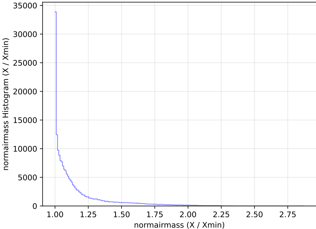
too_elab_r64_d2_griz_v3.4_10yrs WFD g band: normairmass Histogram
