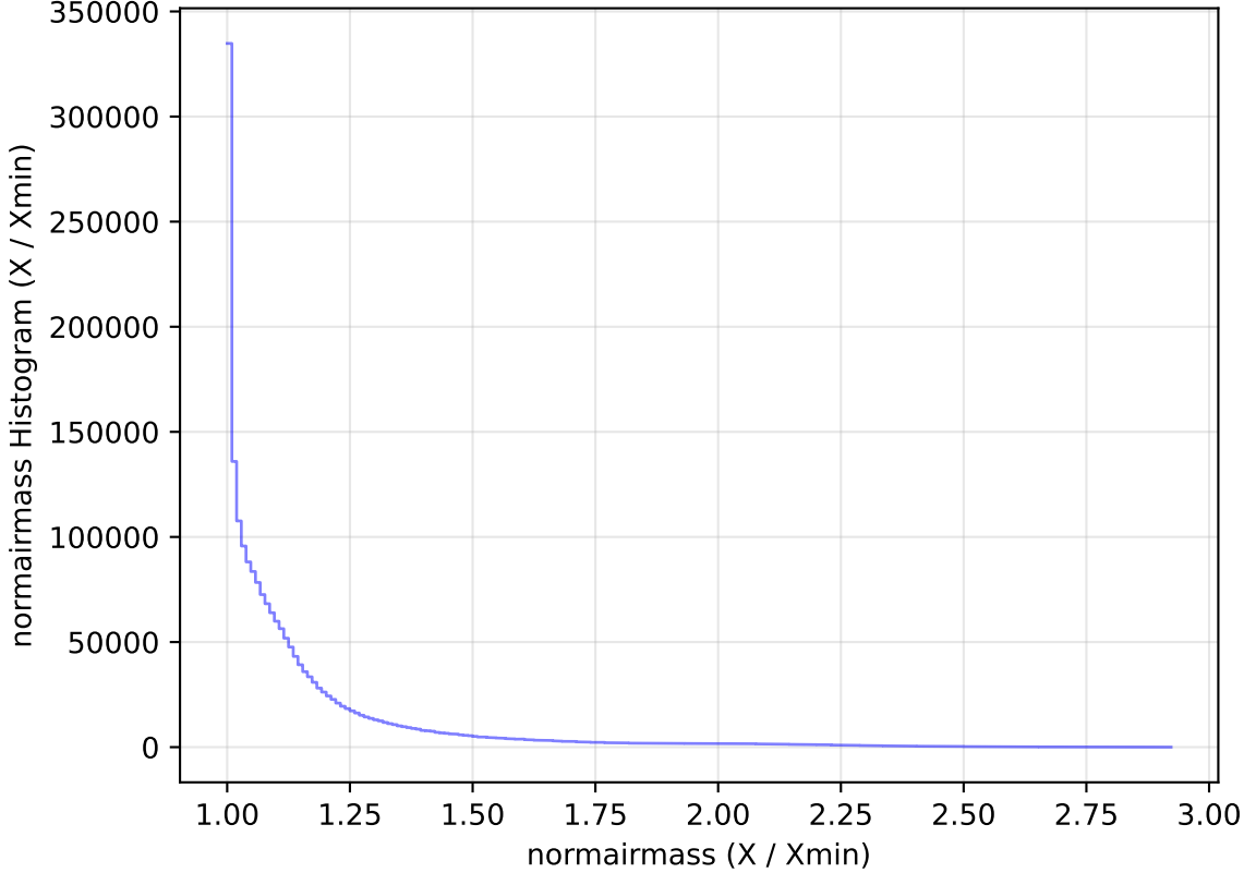
too_elab_r64_d2_griz_v3.4_10yrs WFD all bands: normairmass Histogram
