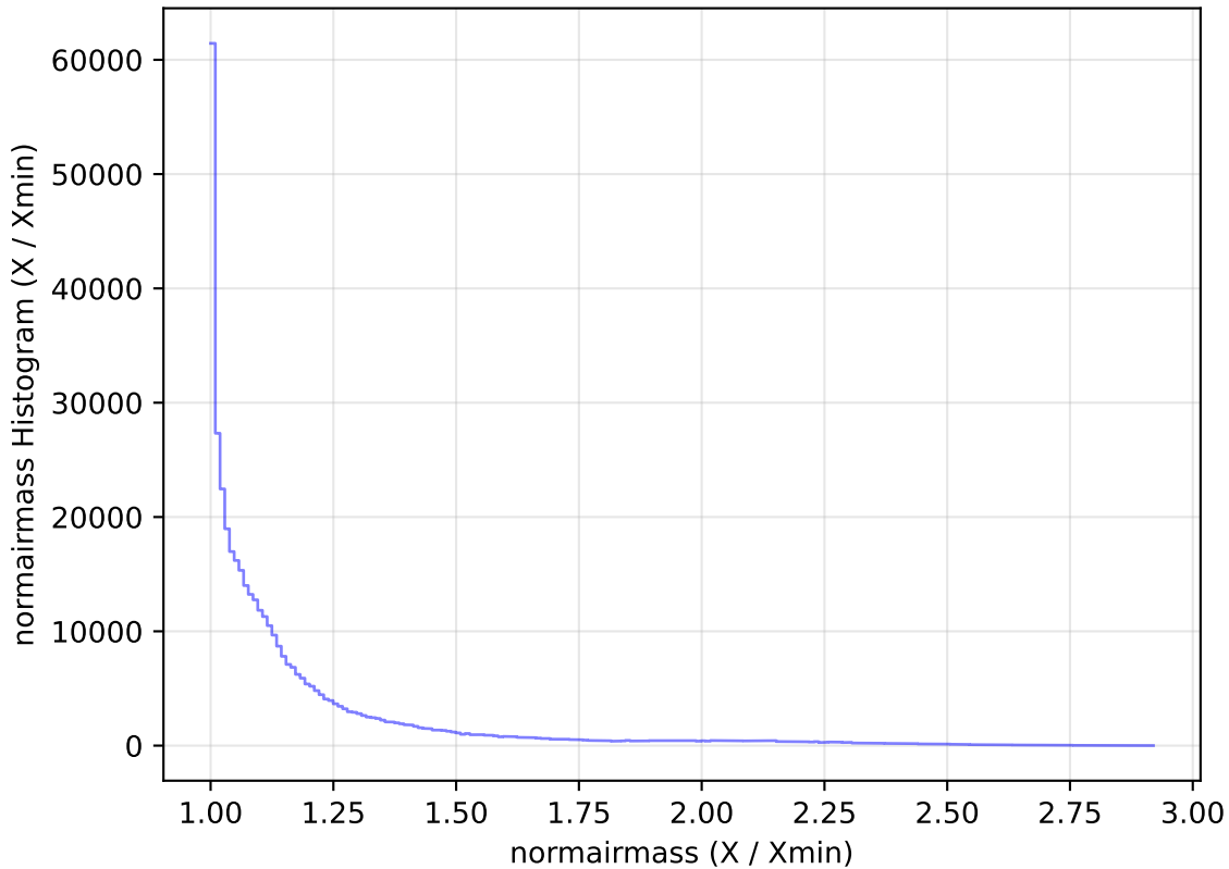
too_elab_r64_d2_griz_v3.4_10yrs All sky z band: normairmass Histogram
