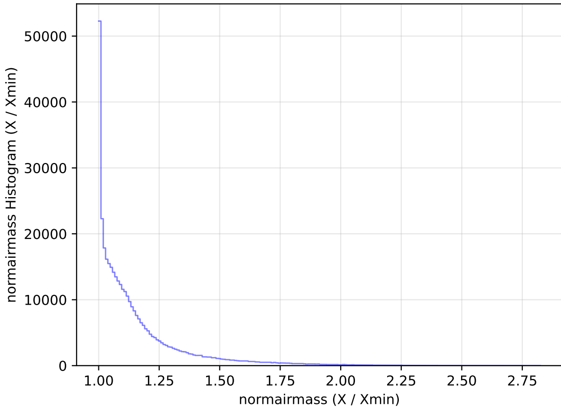
too_elab_r64_d2_griz_v3.4_10yrs All sky y band: normairmass Histogram
