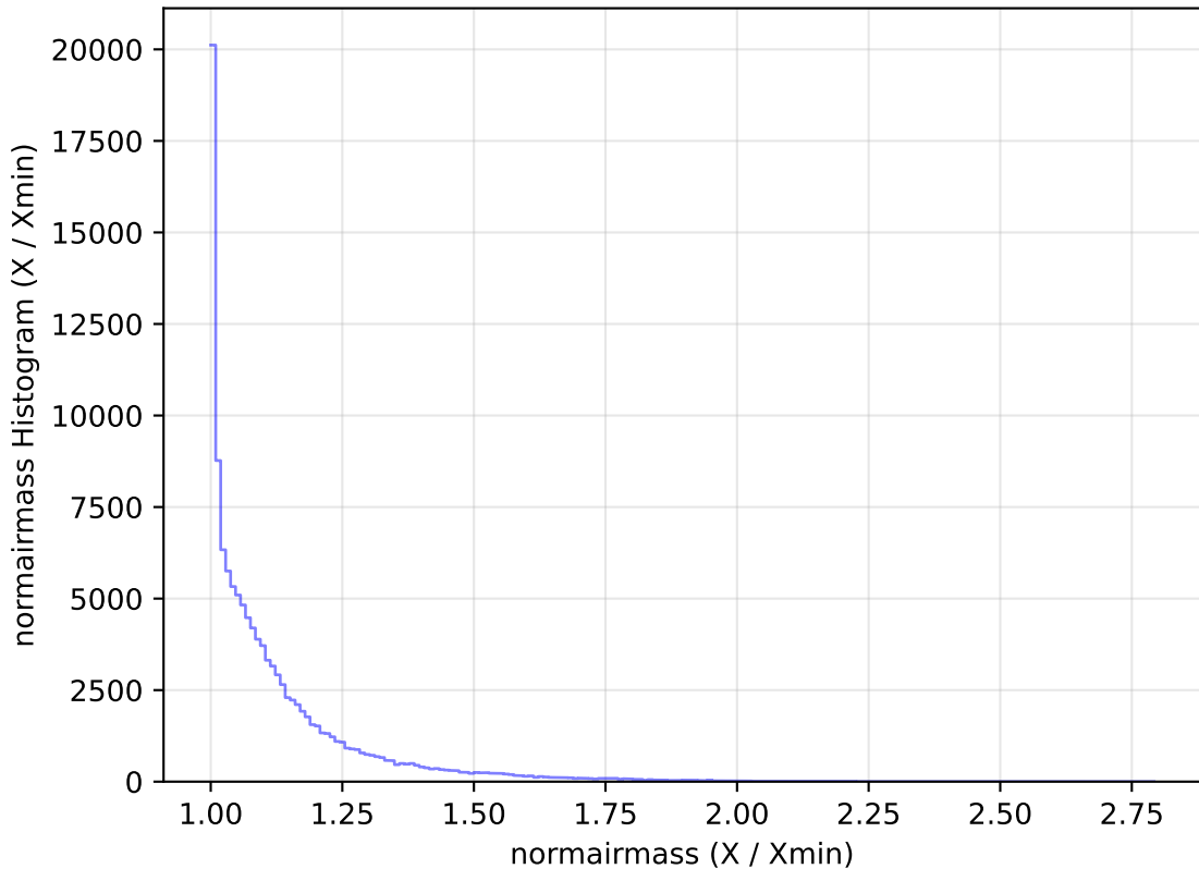
too_elab_r64_d2_griz_v3.4_10yrs All sky u band: normairmass Histogram
