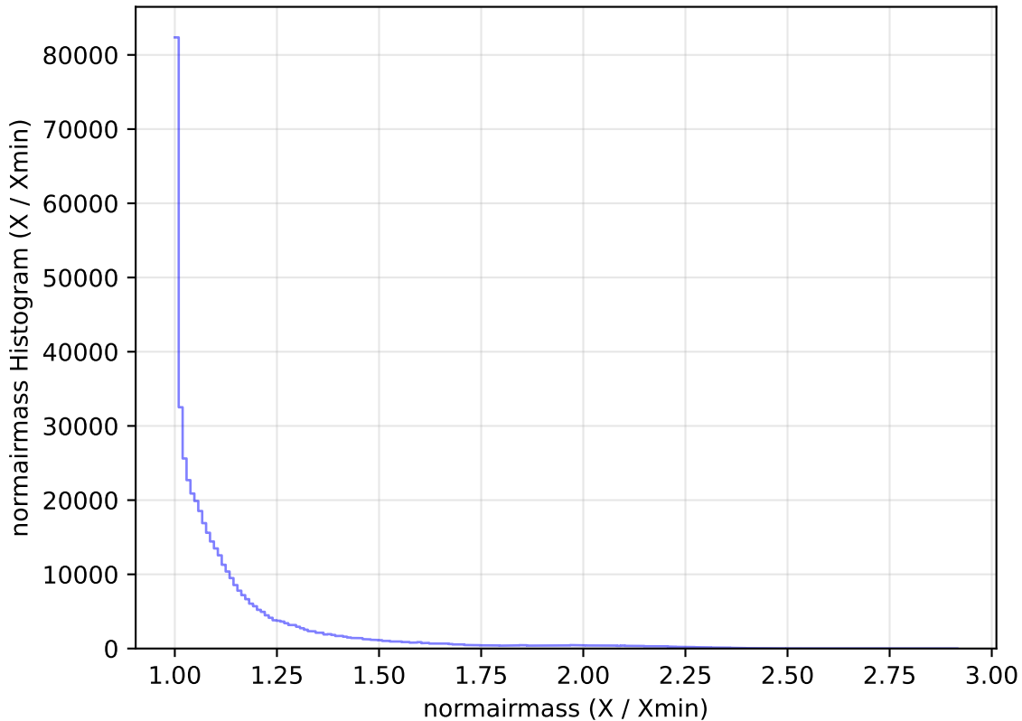
too_elab_r64_d2_griz_v3.4_10yrs All sky r band: normairmass Histogram
