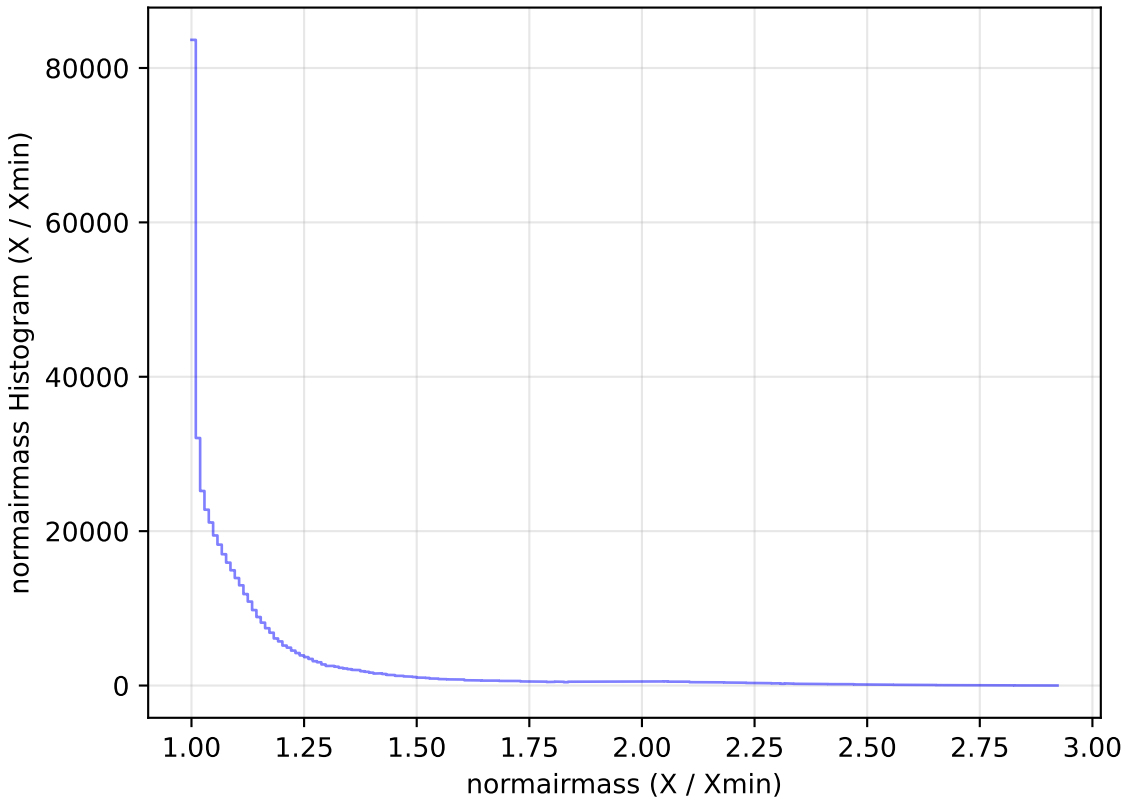
too_elab_r64_d2_griz_v3.4_10yrs All sky i band: normairmass Histogram
