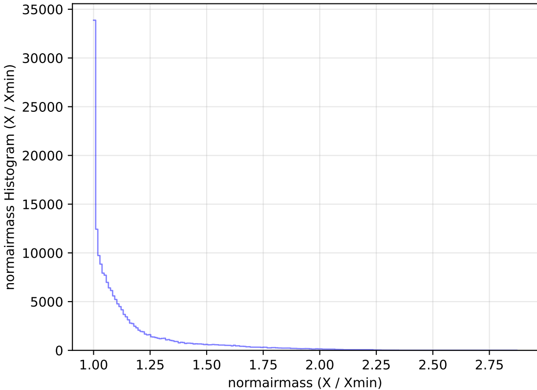
too_elab_r64_d2_griz_v3.4_10yrs All sky g band: normairmass Histogram
