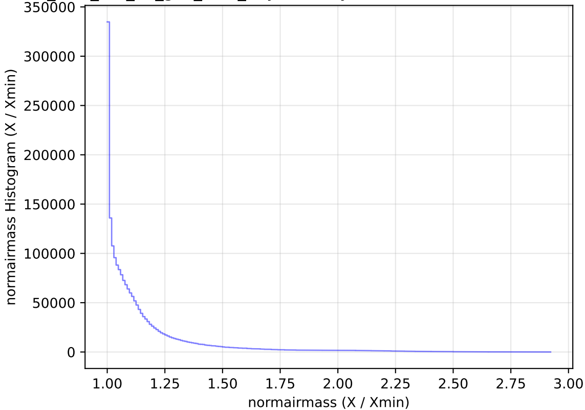
too_elab_r64_d2_griz_v3.4_10yrs All sky all bands: normairmass Histogram
