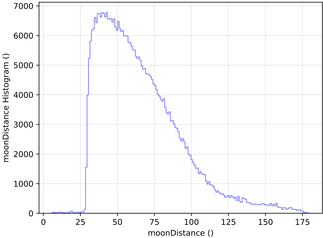
too_elab_r64_d2_griz_v3.4_10yrs WFD y band: moonDistance Histogram
