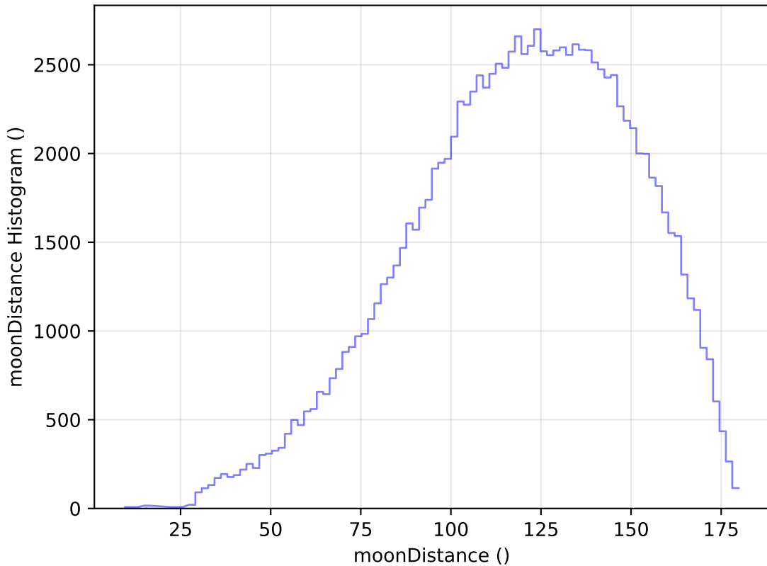
too_elab_r64_d2_griz_v3.4_10yrs WFD u band: moonDistance Histogram
