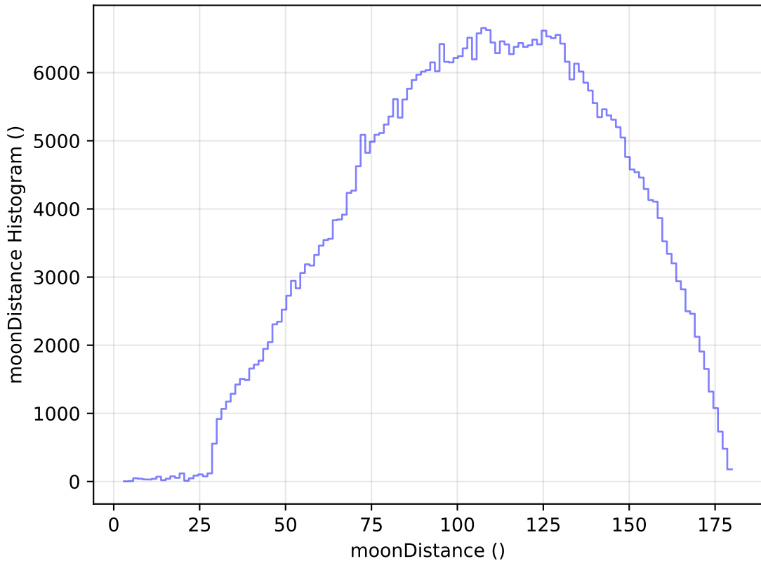
too_elab_r64_d2_griz_v3.4_10yrs WFD r band: moonDistance Histogram
