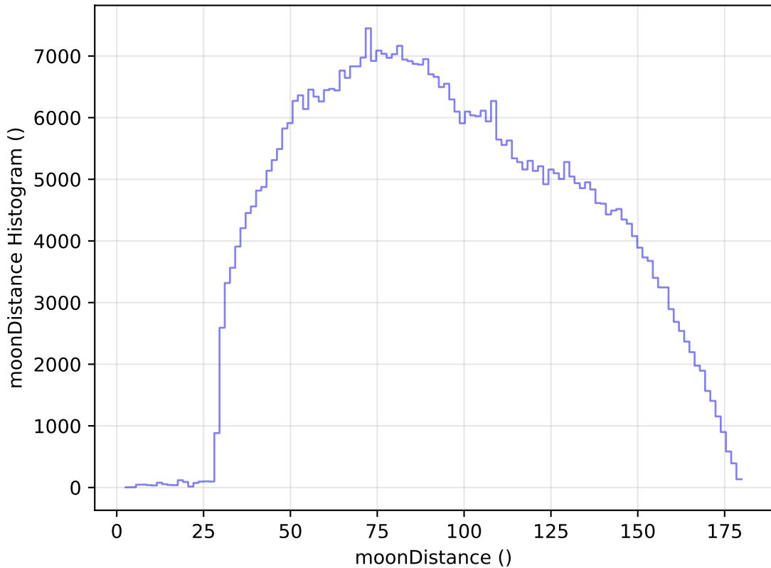
too_elab_r64_d2_griz_v3.4_10yrs WFD i band: moonDistance Histogram
