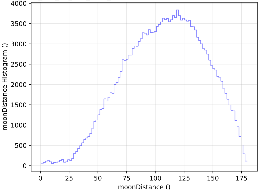
too_elab_r64_d2_griz_v3.4_10yrs WFD g band: moonDistance Histogram
