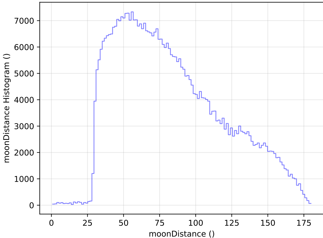
too_elab_r64_d2_griz_v3.4_10yrs All sky z band: moonDistance Histogram
