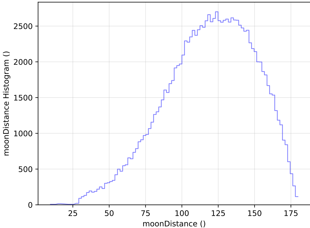
too_elab_r64_d2_griz_v3.4_10yrs All sky u band: moonDistance Histogram
