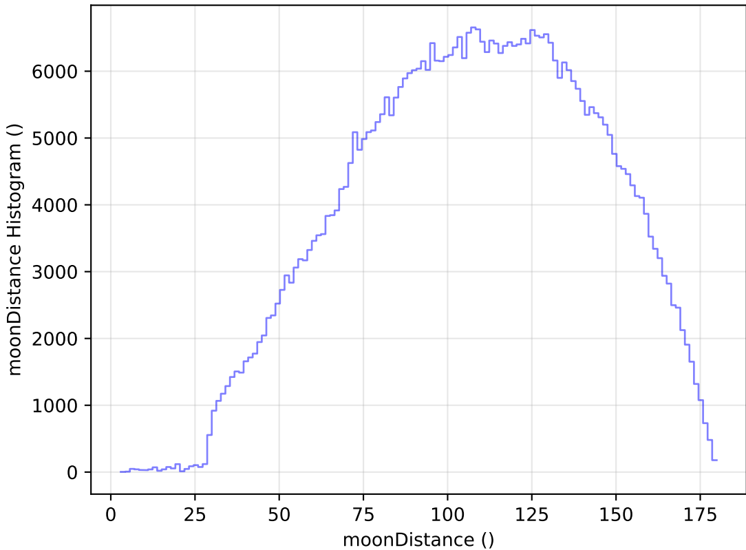
too_elab_r64_d2_griz_v3.4_10yrs All sky r band: moonDistance Histogram
