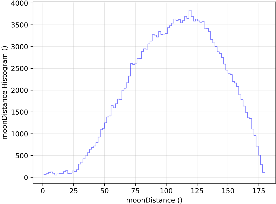
too_elab_r64_d2_griz_v3.4_10yrs All sky g band: moonDistance Histogram
