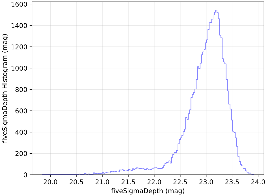
too_elab_r64_d2_griz_v3.4_10yrs Yr 1 z band: fiveSigmaDepth Histogram
