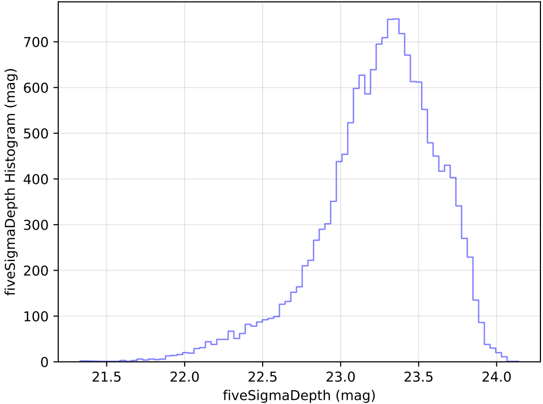
too_elab_r64_d2_griz_v3.4_10yrs Yr 1 u band: fiveSigmaDepth Histogram
