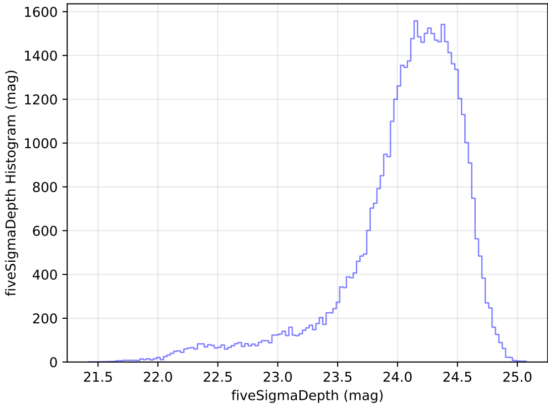
too_elab_r64_d2_griz_v3.4_10yrs Yr 1 r band: fiveSigmaDepth Histogram
