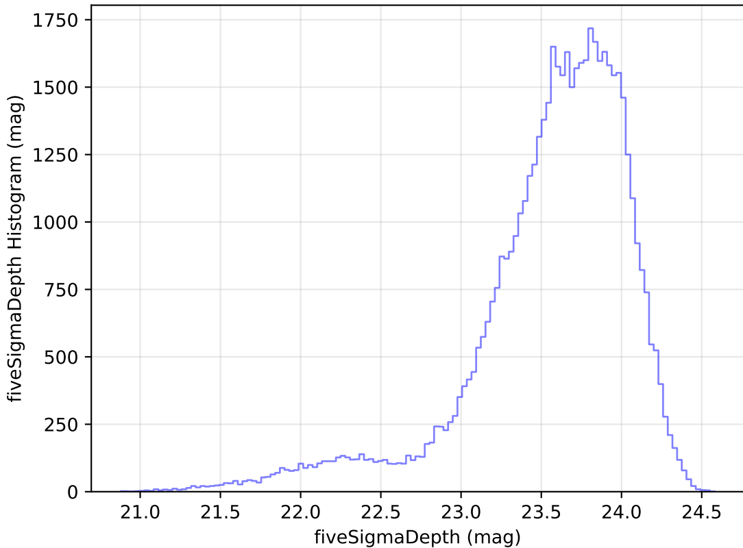
too_elab_r64_d2_griz_v3.4_10yrs Yr 1 i band: fiveSigmaDepth Histogram
