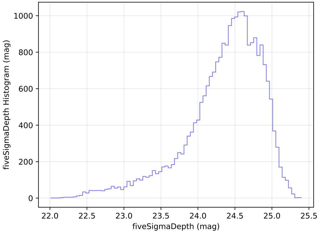
too_elab_r64_d2_griz_v3.4_10yrs Yr 1 g band: fiveSigmaDepth Histogram
