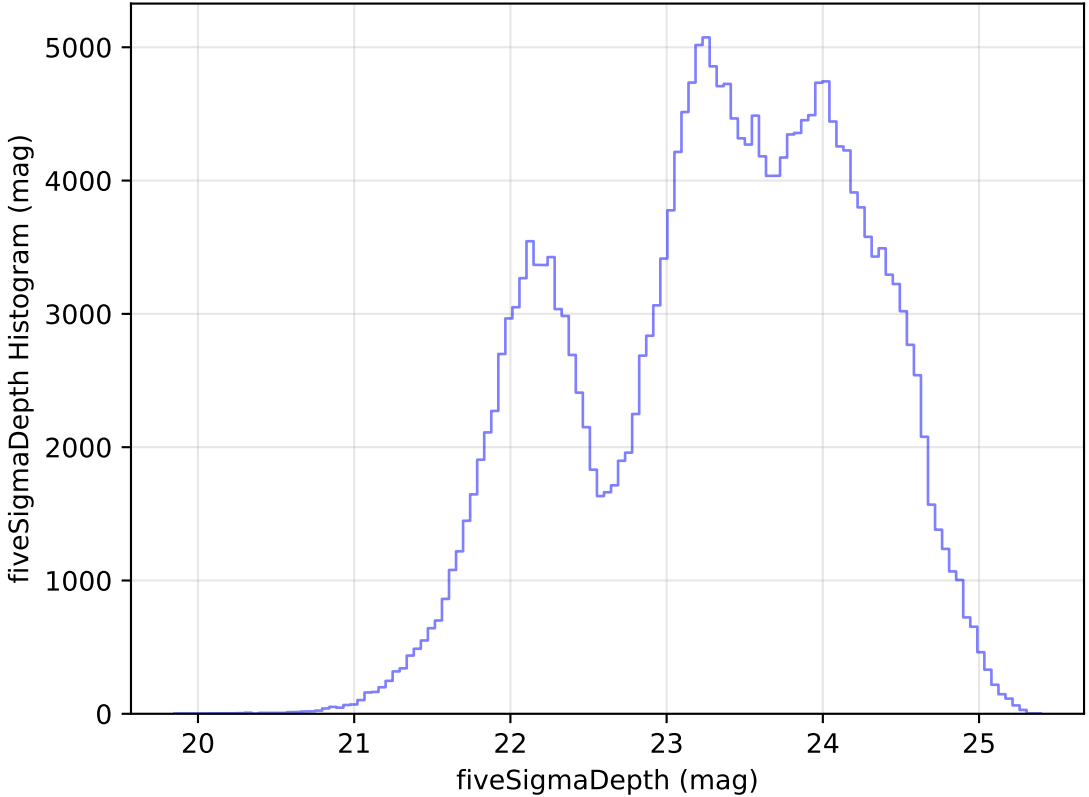
too_elab_r64_d2_griz_v3.4_10yrs Yr 1 all bands: fiveSigmaDepth Histogram
