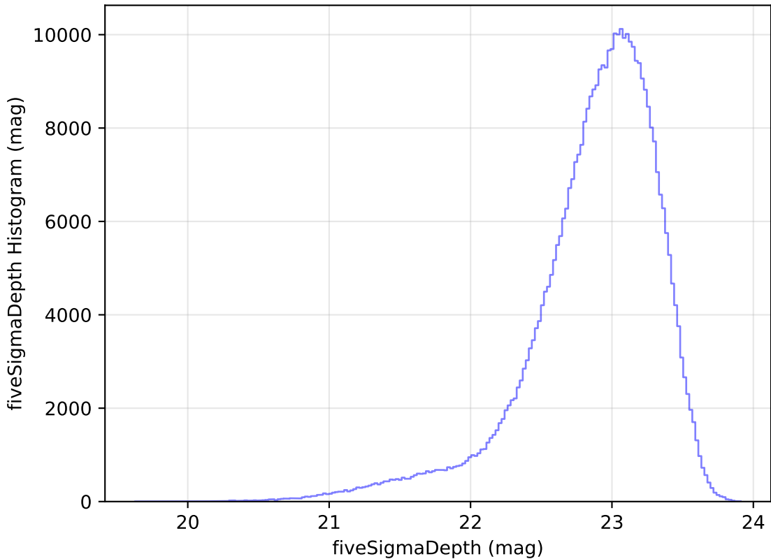
too_elab_r64_d2_griz_v3.4_10yrs WFD z band: fiveSigmaDepth Histogram
