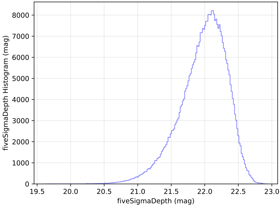
too_elab_r64_d2_griz_v3.4_10yrs WFD y band: fiveSigmaDepth Histogram
