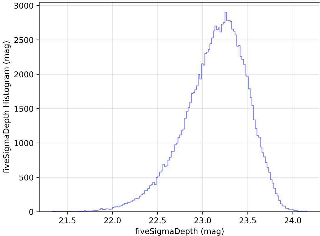
too_elab_r64_d2_griz_v3.4_10yrs WFD u band: fiveSigmaDepth Histogram
