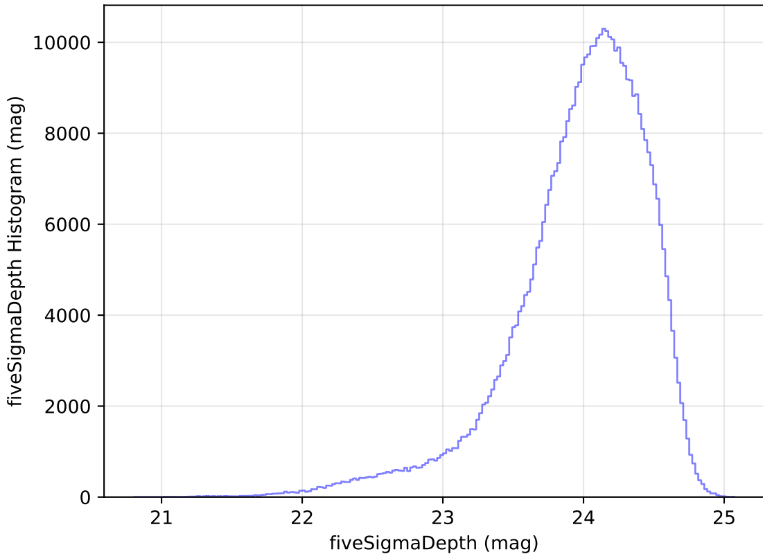
too_elab_r64_d2_griz_v3.4_10yrs WFD r band: fiveSigmaDepth Histogram
