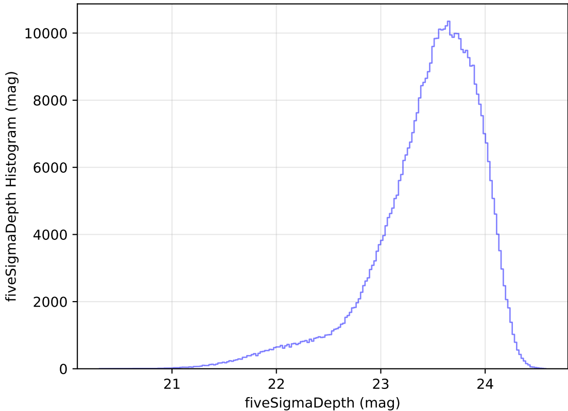
too_elab_r64_d2_griz_v3.4_10yrs WFD i band: fiveSigmaDepth Histogram
