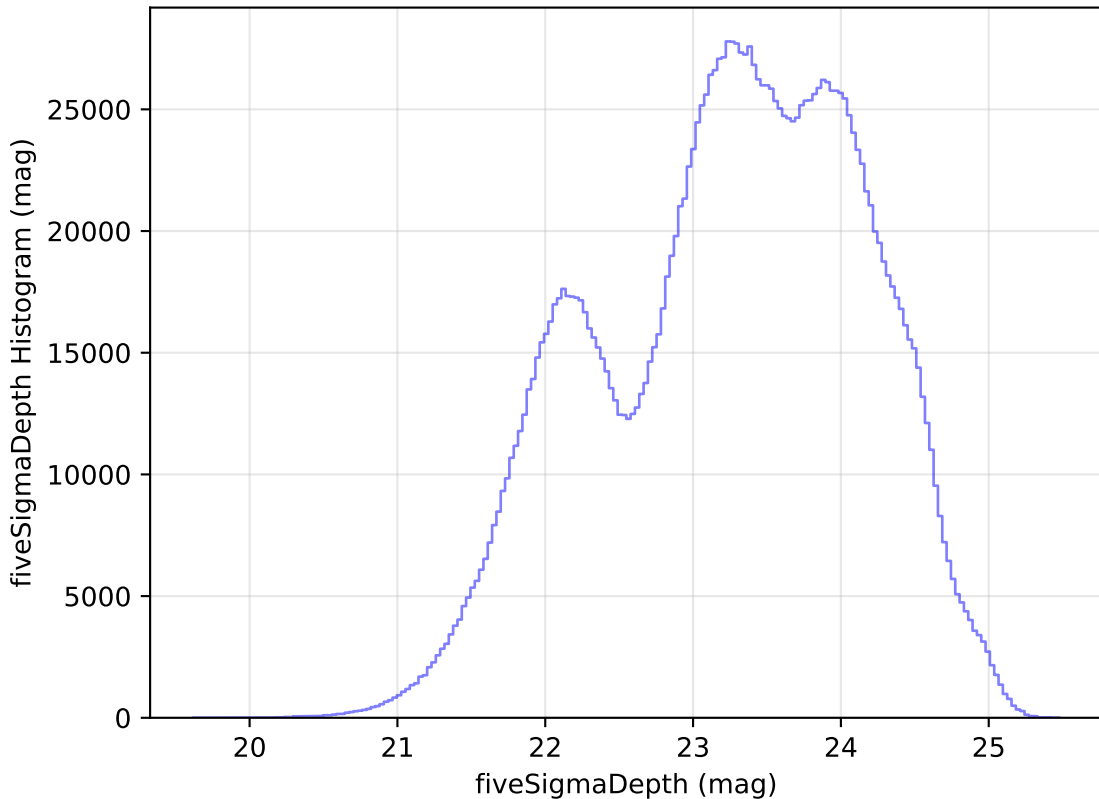
too_elab_r64_d2_griz_v3.4_10yrs WFD all bands: fiveSigmaDepth Histogram
