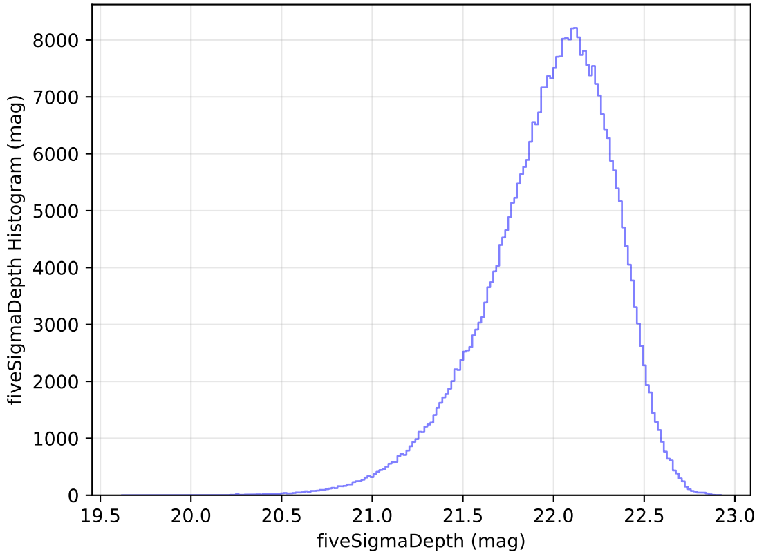
too_elab_r64_d2_griz_v3.4_10yrs All sky y band: fiveSigmaDepth Histogram
