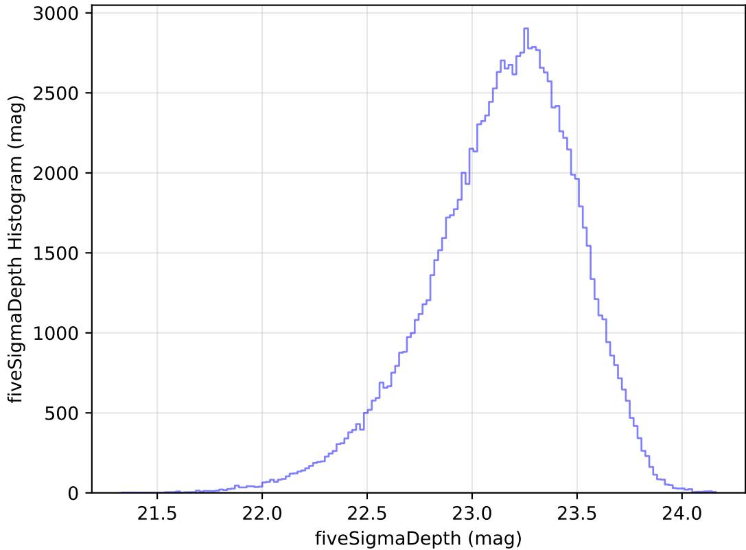
too_elab_r64_d2_griz_v3.4_10yrs All sky u band: fiveSigmaDepth Histogram
