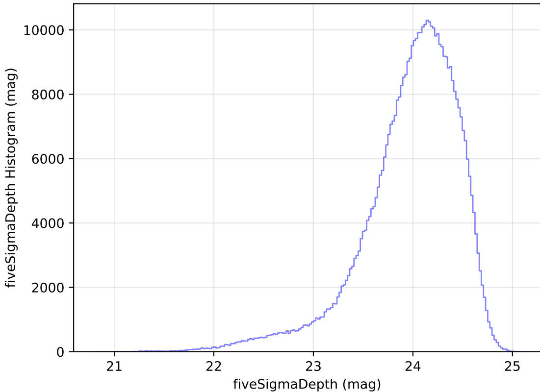
too_elab_r64_d2_griz_v3.4_10yrs All sky r band: fiveSigmaDepth Histogram
