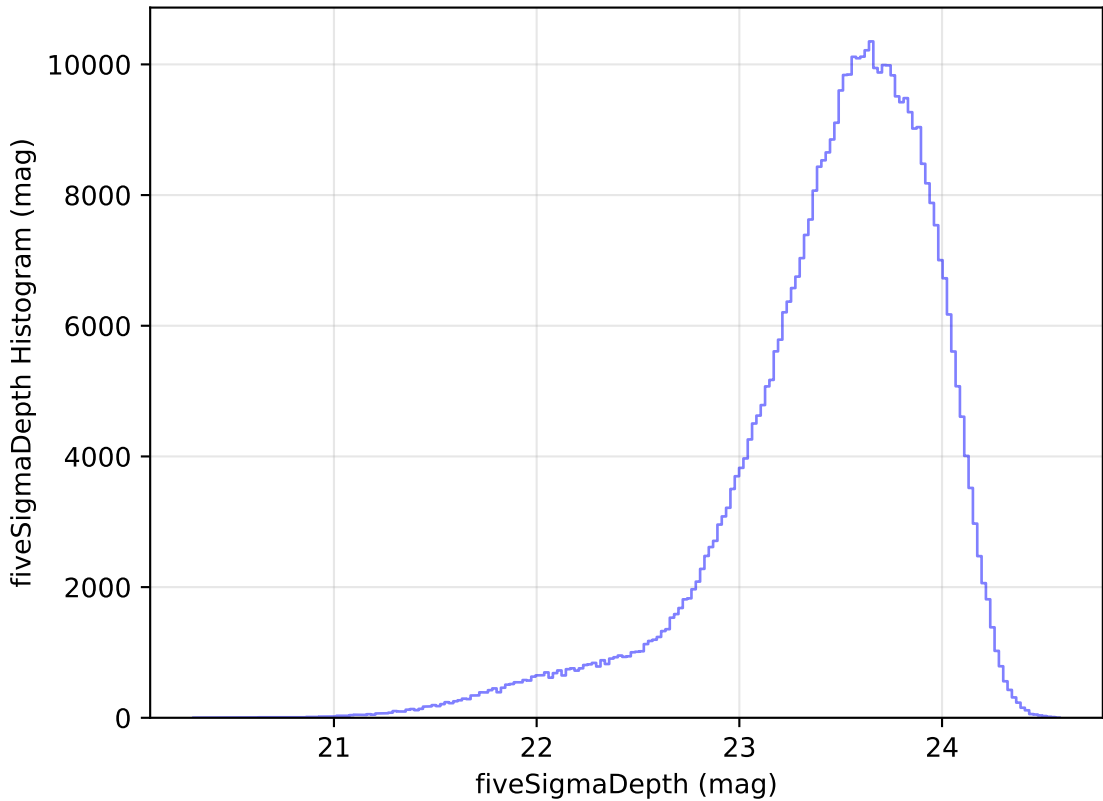
too_elab_r64_d2_griz_v3.4_10yrs All sky i band: fiveSigmaDepth Histogram
