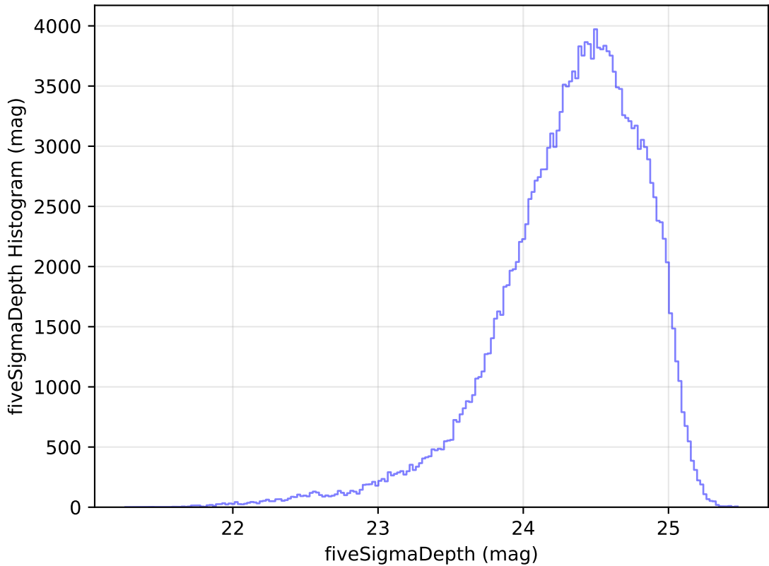
too_elab_r64_d2_griz_v3.4_10yrs All sky g band: fiveSigmaDepth Histogram
