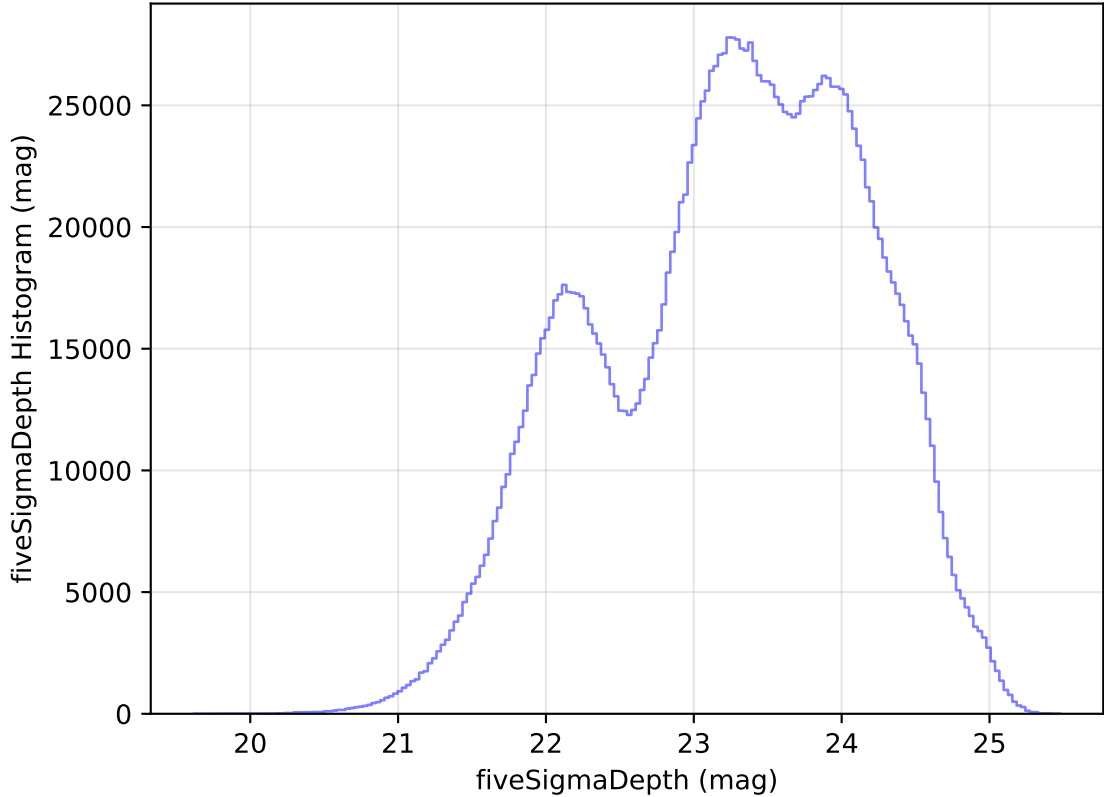
too_elab_r64_d2_griz_v3.4_10yrs All sky all bands: fiveSigmaDepth Histogram
