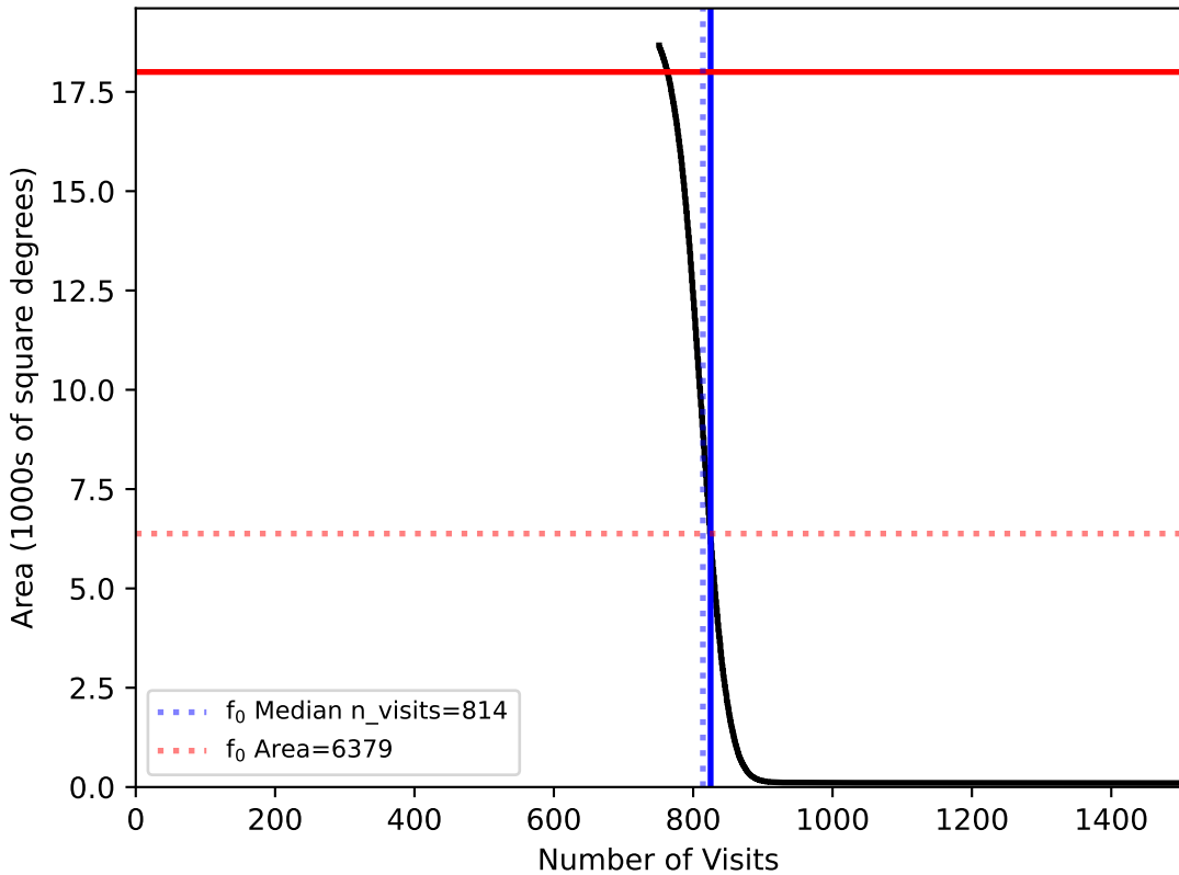
too_elab_r64_d2_griz_v3.4_10yrs WFD: fO
