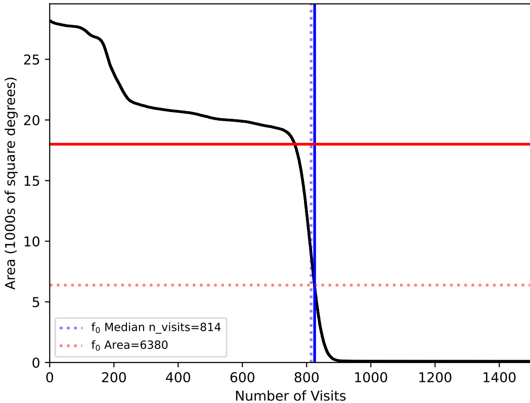
too_elab_r64_d2_griz_v3.4_10yrs All sky: fO
