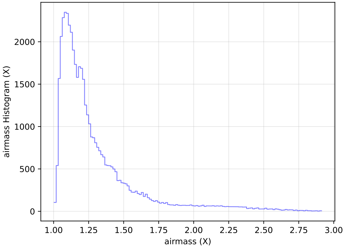
too_elab_r64_d2_griz_v3.4_10yrs Yr 1 z band: airmass Histogram
