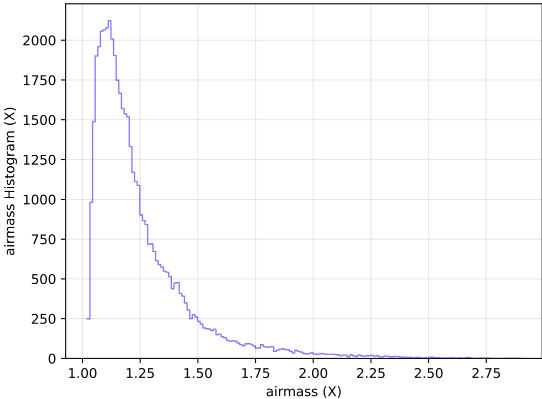
too_elab_r64_d2_griz_v3.4_10yrs Yr 1 y band: airmass Histogram
