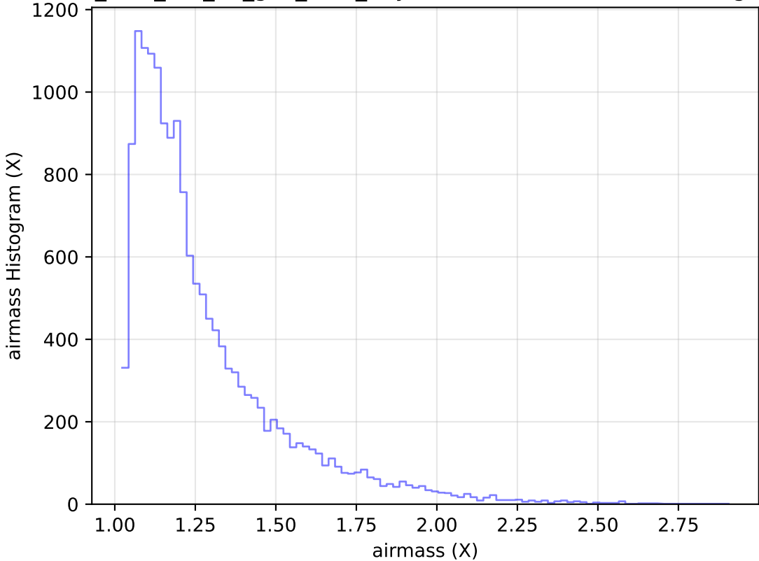
too_elab_r64_d2_griz_v3.4_10yrs Yr 1 u band: airmass Histogram
