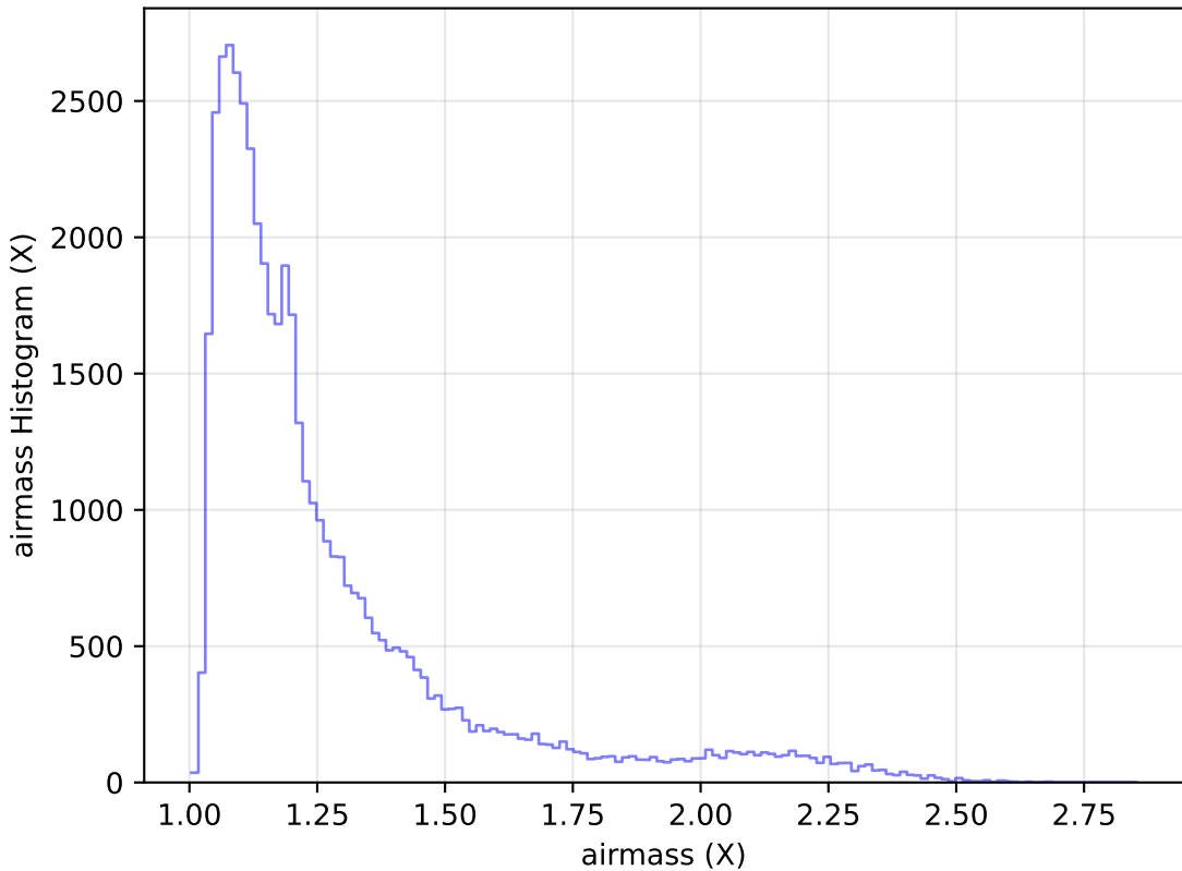
too_elab_r64_d2_griz_v3.4_10yrs Yr 1 r band: airmass Histogram
